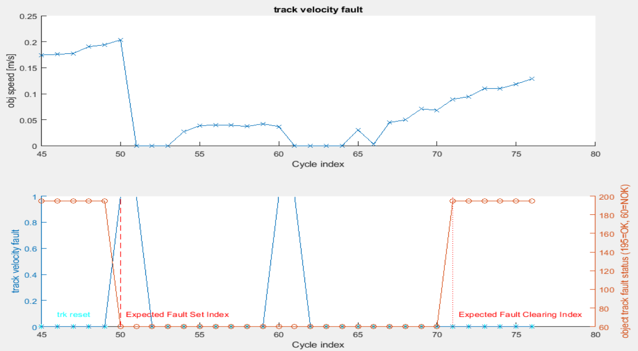
Test Case (18): Obj_Velocity_Output_Fault
